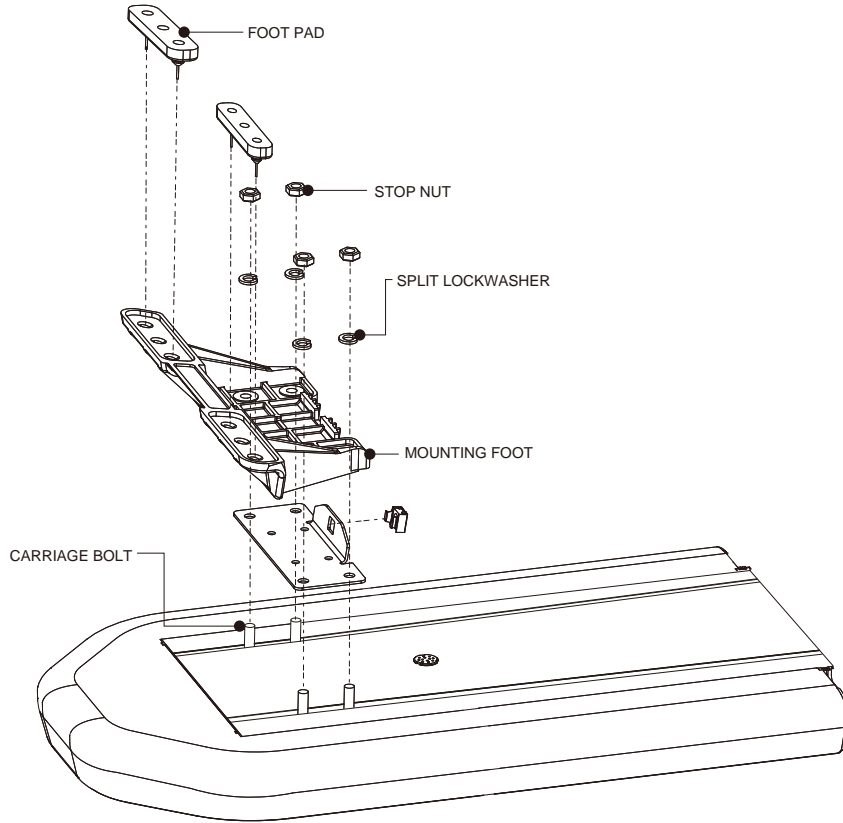
Upside down view of lightbar with mounting foot
